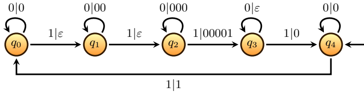
Fig. 5: A finite state transducer that realises the mass product and displacement given in Example 10 on the corresponding block stream.
