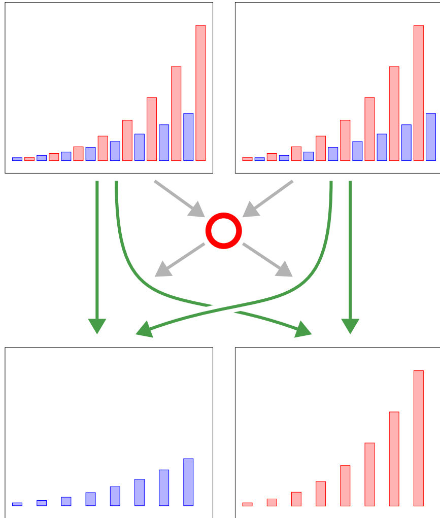
Fig. 8: The graphs illustrate growth of the block size of \sigma_1 (upper left), \sigma_2 (upper right), \tau_1 (lower left) and \tau_2 (lower right). The green arrows stand for finite state transductions, while the red circle and the grey arrows represent impossible transductions.
