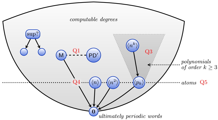
Fig. 2: The partial order of Transducer degrees. Some open problems are indicated in red: Q1, \dots, Q5 refer to open problems 1, ..., 5, respectively. The blue nodes are degrees. Note that \langle n \rangle and \langle n^2 \rangle are atoms, while \langle n^k \rangle is not an atom for k \geq 3 . The notation \langle \cdot \rangle is defined above. Here p_k is a particular polynomial of order k . The degree of \langle p_k \rangle is an atom and all other polynomials of order k can be transduced to \langle p_k \rangle , but not vice versa.
