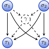
Fig. 7: Construction to show that there are pairs of degrees without supremum, and pairs of degrees without infimum.
