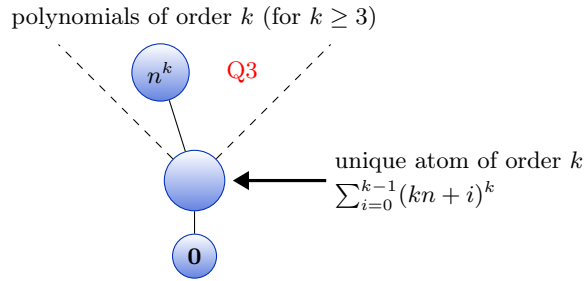
Fig. 3: Structure of degrees of polynomials of order k \geq 3 . The node Q3 points to open problem 3 concerning the view on this part of the degree structure.
